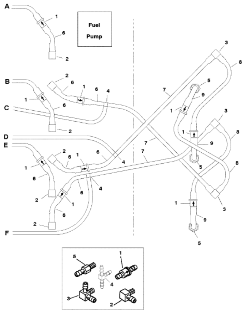
A THRU F = TUBING IS CONTINUED ON STARBOARD SIDE
